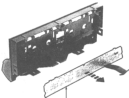
Step 9 Remove the operation P.C.B..
